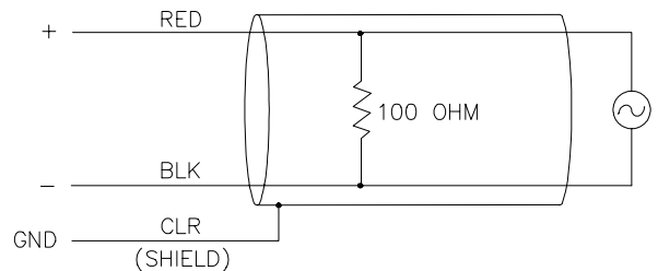
Figure 1. LI200S Schematic
